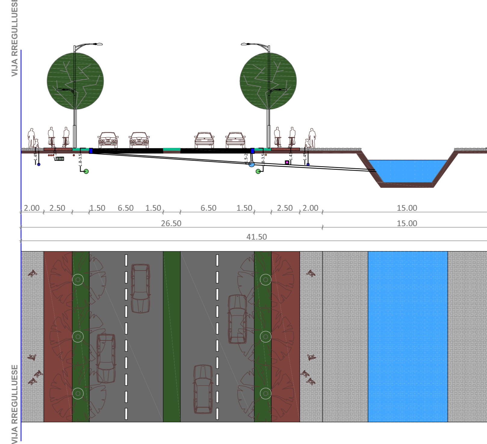
RRUGA MBI LUMIN E HAPUR "PRISHTINA" (H-H)
